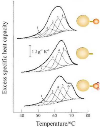
DSC traces of glucoamylase
